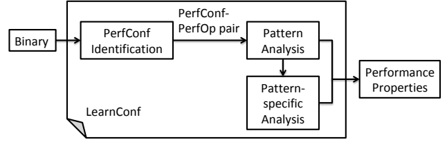
Figure 2. LearnConf Overview
